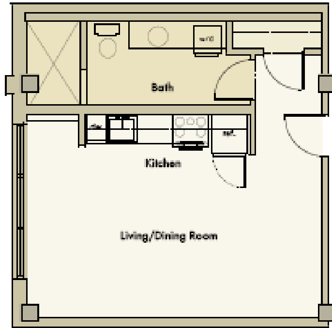
Loft 14 1/4" = 1'-0"
